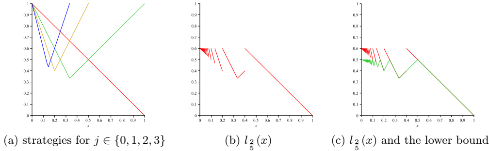
FIG. 4.2. More ‘zigzag’ functions.
