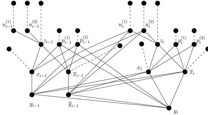
FIG. 3.2. Connections of G_{i-1}(\nabla) and G_i(\exists) .
