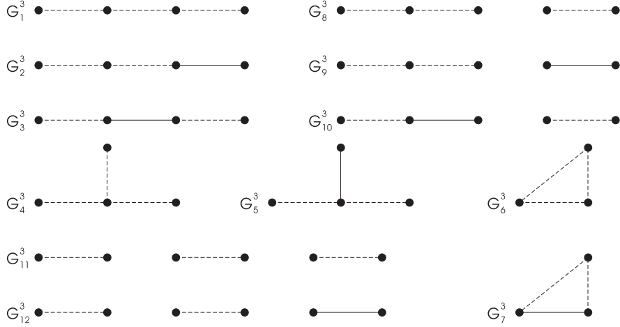
FIGURE 2. Coloured graphs with three edges
