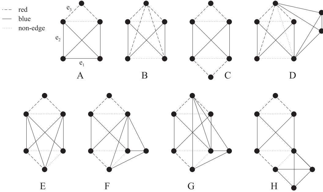
FIGURE 3. Desired subgraphs
