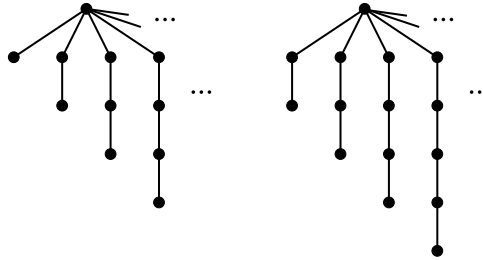
Fig. 1. Each of the two graphs is a subgraph of the other.
