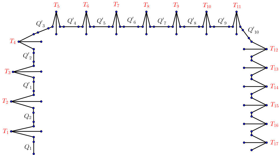
Fig. 1. A sketch of the tree T(X) .
