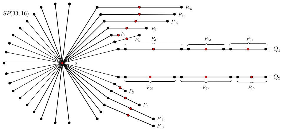
Fig. 2. A sketch of the tree G .
