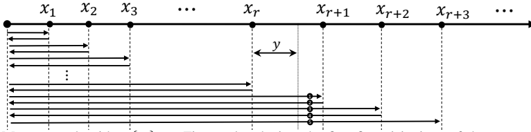
Fig. 1 Monotone algorithm \{x_i\}_{i \geq 1} . Figure also depicts the first five visitations of the treasure that is placed at x_r + y .
