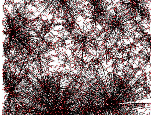
Figure 1: A simulation of the GEO-P model, with n = 5,000 , \alpha = 0.7 , \beta = 0.15 , m = 2 , and p = 0.9 .
